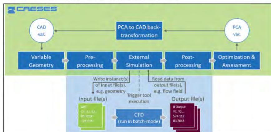
Figure 2 - PCA based SDD process as realised with CAESES
