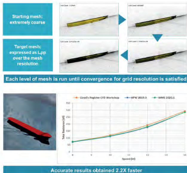
Figure 2: MMS automatically refines the mesh based on the flow field until a target mesh is met
