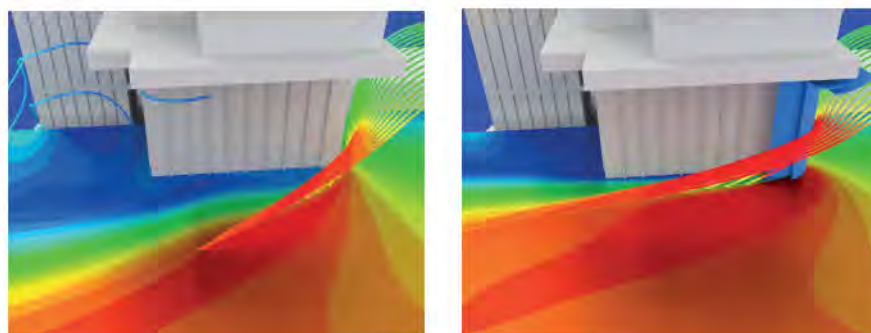
Fig. 3: "Improvement of corner flow on the front edge of the deckhouse using deflector blades"
