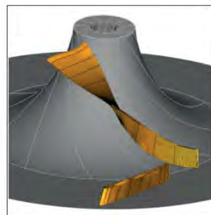
Figure 4 - Compressor main blade and diffuser vane with discretisation points used for the PCA
