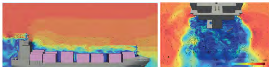
Fig. 1: "Instantaneous turbulent flow field in a vertical plane at center line ( vxz left) and in a horizontal plane 20m above baseline through the deckhouse ( vxy right), obtained from a DES-simulation."
