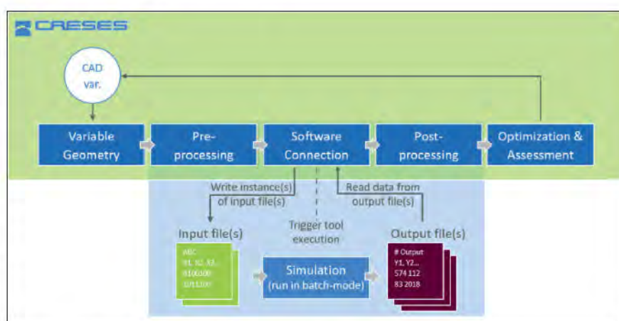
Figure 1 - Standard simulation-driven design process realised with CAESSES
