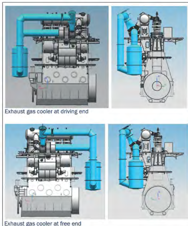
Exhaust gas cooler at free end
